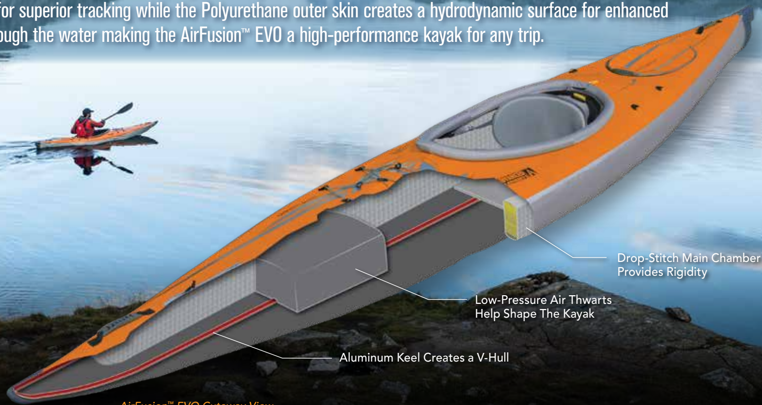
AirFusion™ EVO Cutaway View
